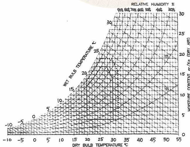
FIGURE Suggested boundaries of outdoor temperature and humidity within which indoor comfort can be provided by natural ventilation. Assumed air speed 2 m/s.
