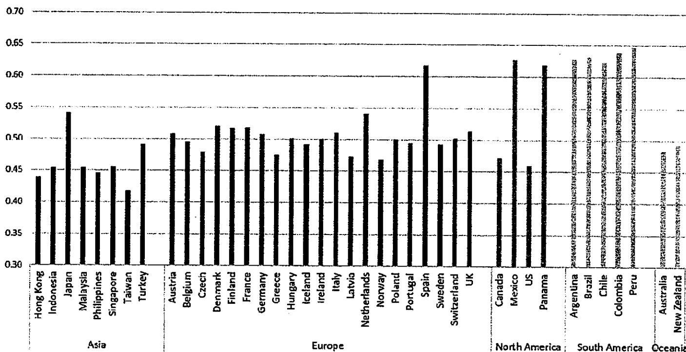
Fig. 1. Stream-weighted average valence of top-200 songs by geographical region and country. This figure plots the average daily stream-weighted average valence (SWAV) per country over our sample period from January 1, 2017, to December 31, 2020. The 40 countries in our sample are grouped by geographical region.
